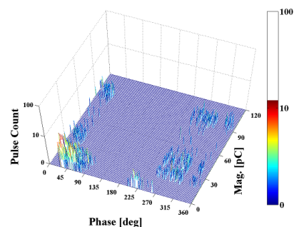
Figure 2. The partial discharge in sample A after 10000 applied impulses, measured at 18 kV, 60 Hz
